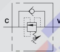
SCHEMA IDRAULICO HYDRAULIC DIAGRAM
